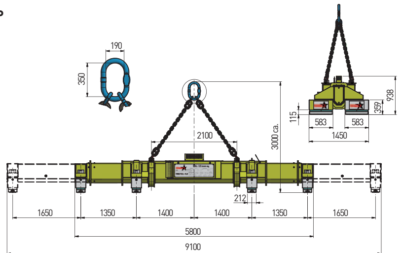
TECHNICAL FEATURES OF THE TELESCOPIC BEAMS "TRETTEL"
